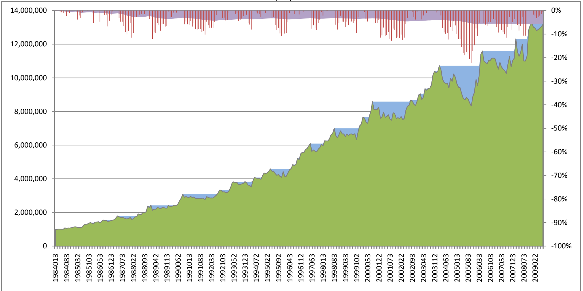
Equity Curve
