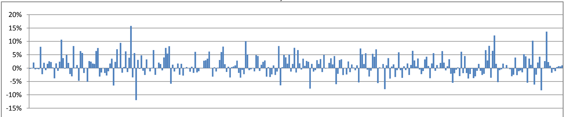
Monthly Returns
